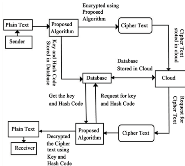
Figure 9: System Flow
