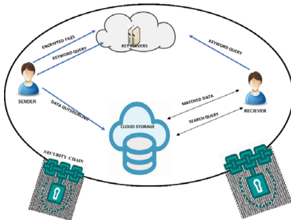
Figure 8: Architecture
