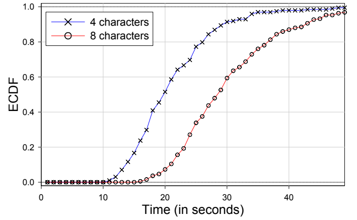
Fig. 8. Empirical CDF of the time it takes for inputting passwords of two different lengths in our protocol. The total numbers of successful trials are 198 (4 characters) and 192 (8 characters).
