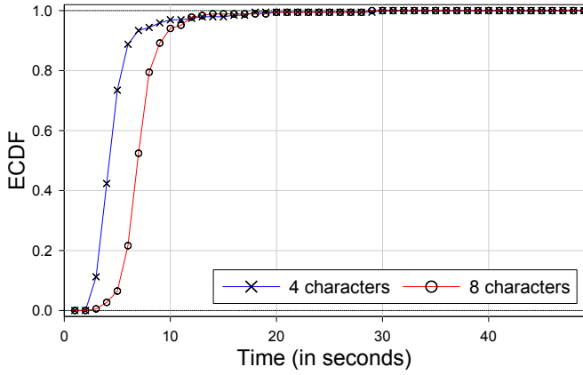
Fig. 6. Empirical CDF of the time it takes for inputting passwords of two different lengths. The total numbers of successful trials are 196 (4 characters) and 185 (8 characters). The keyboard used for input is a qwerty keyboard, which is the typical Android phone keyboard.
