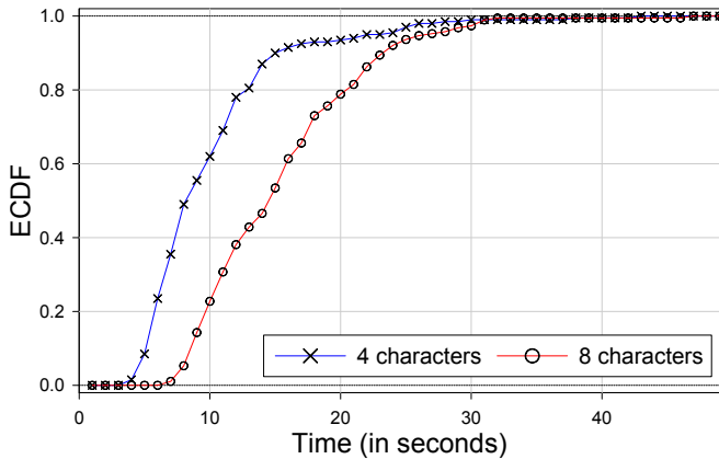
Fig. 7. Empirical CDF of the time it takes for inputting passwords of two different lengths. The total numbers of successful trials are 200 (4 characters) and 189 (8 characters). The keyboard used for input is the a randomized Android phone keyboard (same keyboard is rendered on the smartphone and terminal).
