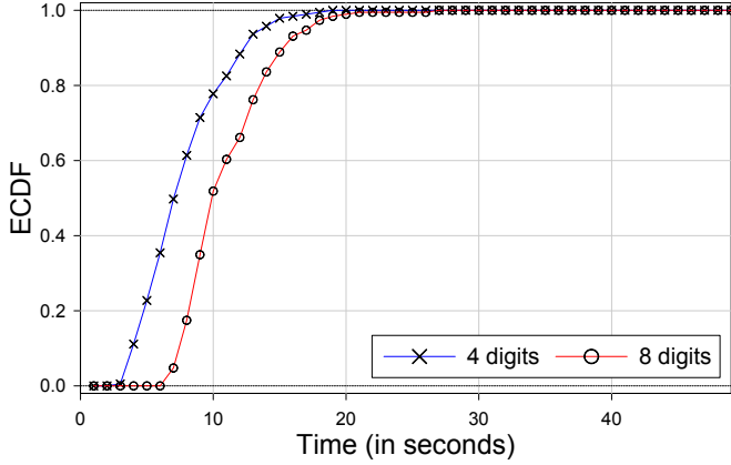
Fig. 5. Empirical CDF of the time it takes for inputting PINs of two different lengths in Protocol 2. The total numbers of successful trials are 189 (4 digits) and 189 (8 digits).
