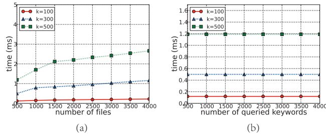
Figure 9: (a) The time to select the top- k files’ identifiers on different scale of file sets. (b) The time to select the top- k files’ identifiers for different number of queried keywords, the number of files in the file set is n = 500 .
