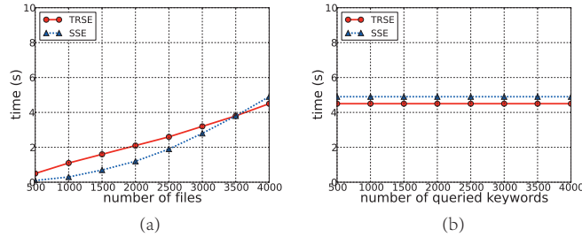
Figure 7: (a) The time to calculate scores on different scale of file sets, the number of keywords in the keyword set is 1000. (b) The time to calculate scores for different number of queried keywords, here the number of files in the file set is n = 4000 .
