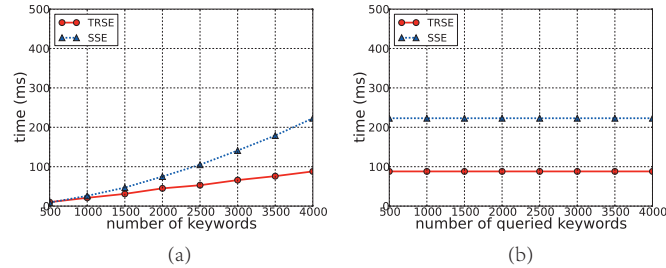
Figure 6: (a) The time to generate trapdoor on different scale of keyword sets. (b) The time to generate trapdoor for different number of queried keywords, the number of keywords in the keyword set is l = 4000 .
