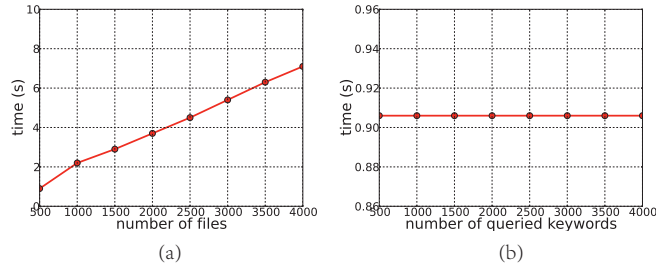
Figure 8: (a) The time to decrypt the result vector on different scale of file sets. (b) The time to decrypt the result vector for different number of queried keywords, the number of files in the file set is n = 500 .
