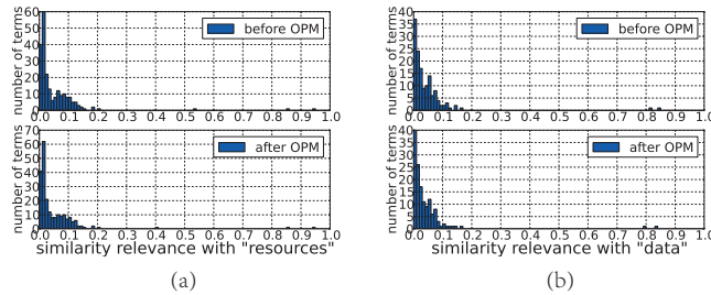
Figure 3: Distribution of similarity relevance of (a) 218 terms with “resources” before and after OPM in the NSF file set. (b) 142 terms with “data” before and after OPM in the 20 Newsgroups data set.
