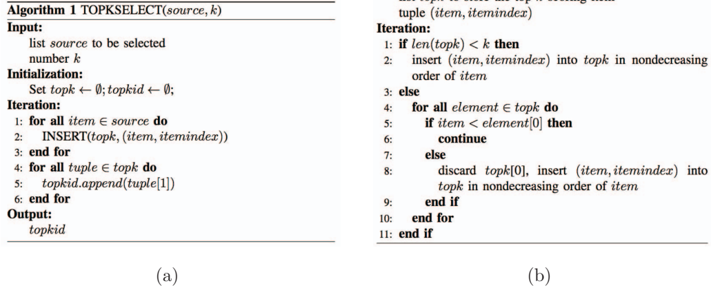
Figure 4: (a) Algorithm TOPKSELECT. (b) Algorithm INSERT.
