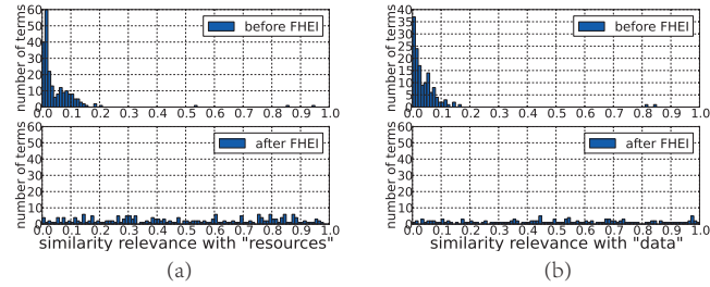
Figure 5: Distribution of similarity relevance of (a) 218 terms with “resources” before and after FHEI in the NSF file set. (b) 142 terms with “data” before and after FHEI in the 20 Newsgroups data set.
