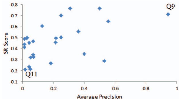
Fig. 5. Average precision versus SR score for queries on INEX using PRMS, K = 20 and (\gamma_A, \gamma_T, \gamma_S) = (1, 0.3, 0.5) .
