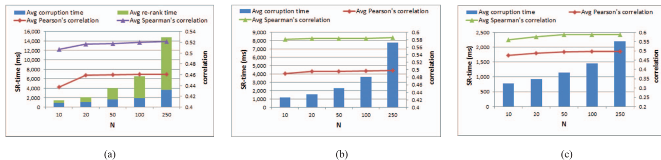
Fig. 9. Approximations on SemSearch: (a) QAO-Approx. (b) SGS-Approx. (c) Combination of QAO and SGS.
