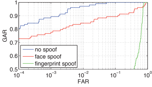
Fig. 4. ROC curves of the considered multimodal biometric system, under a simulated spoof attack against the fingerprint or the face matcher.
