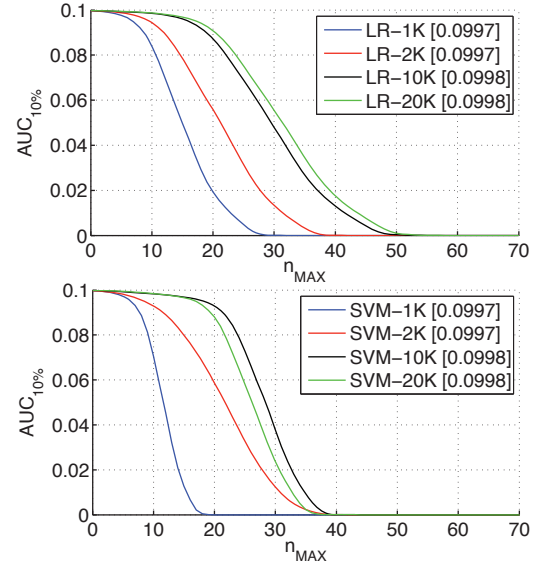
Fig. 3. \text{AUC}_{10\%} attained on TS as a function of n_{\text{max}} , for the LR (top) and SVM (bottom) classifier, with 1,000 (1K), 2,000 (2K), 10,000 (10K) and 20,000 (20K) features. The \text{AUC}_{10\%} value for n_{\text{max}} = 0 , corresponding to classical performance evaluation, is also reported in the legend between square brackets.
