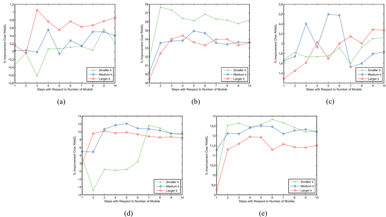
Fig. 1. Average relative improvement of GLE over RAKEL in terms of five different evaluation metrics with respect to different parameters k and M : (a) Hamming loss. (b) Ranking loss. (c) Subset 0/1 loss. (d) One error. (e) Average precision.
