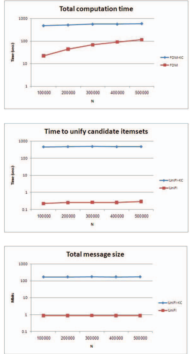
Fig. 1. Computation and communication costs versus the number of transactions N
