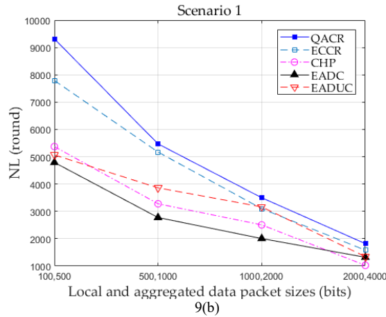
Fig. 9. Steady state and network lifetime (NL) for different packet sizes under the Scenario 1: (a) First node dies (FND), and (b) Network lifetime (NL).
