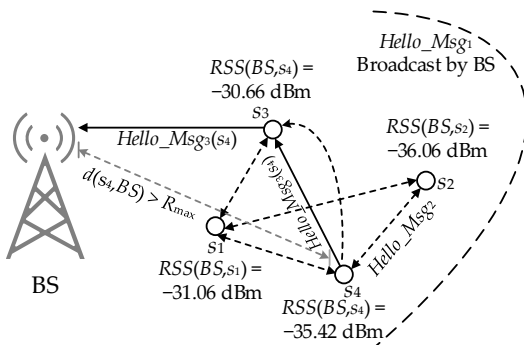
Fig. 2. An example of nodes' information collection and sending to the BS.
