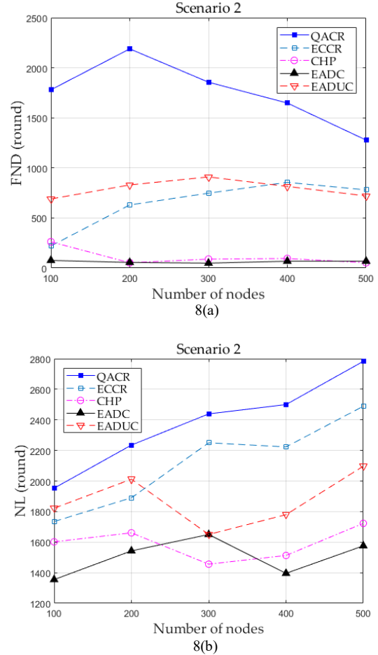
Fig. 8. Steady state and network lifetime (NL) for different number of sensor nodes under the Scenario 2: (a) First node dies (FND), and (b) Network lifetime (NL).
