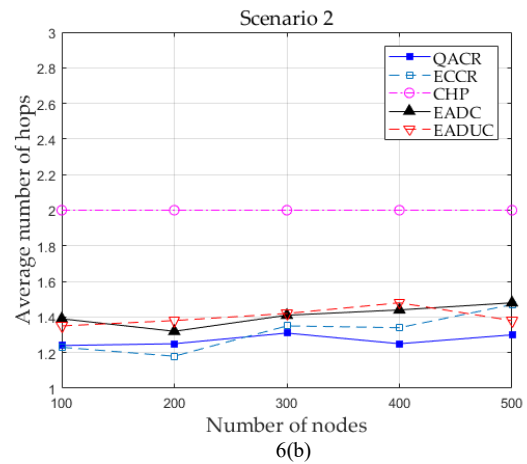
Fig. 6. Average number of hops of the data packets received at the BS for different number of sensor nodes under the scenarios; (a) Scenario 1: random with uniform node distribution, and (b) Scenario 2: random with non-uniform node distribution.
