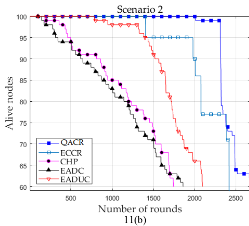
Fig. 11. Steady state and network lifetime (NL) for BS at center under the Scenario 1: and Scenario 2: (a) First node dies (FND), and (b) Network lifetime (NL).
