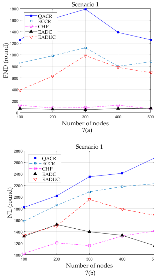
Fig. 7. Steady state and network lifetime (NL) for different number of sensor nodes under the Scenario 1: (a) First node dies (FND), and (b) Network lifetime (NL).
