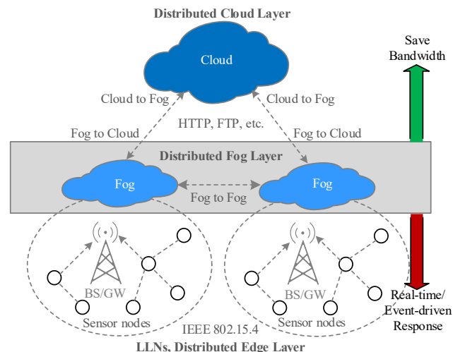
Fig. 1. An example architecture of a Fog-enabled IoT.
