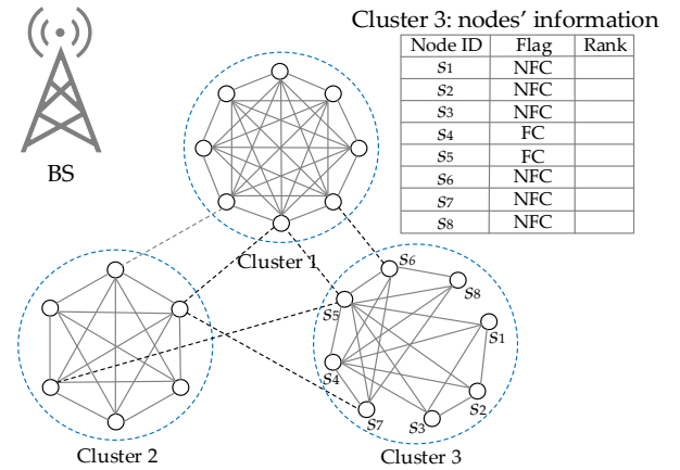
Fig. 3. An example of clustering of the nodes. Case1: all cluster members (CMs) are within the communication range R_n from any other CM (defined by flag = 'FC' ), see Clusters 1 and Cluster 2. Case 2: a set of nodes \{s_1, s_2, s_3\} are out of R_n from some of the CMs (defined by flag = 'NFC' ) and a set \{s_4, s_5\} belongs to an intersection region of two independent sets \{s_1, \dots, s_5\} \cap \{s_4, \dots, s_8\} , see Cluster 3.
