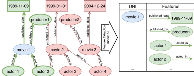
Fig. 3. Feature Extraction using predicate and node in same feature
