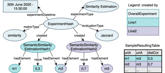
Fig. 2. Sample resulting meta graph from DistSim
