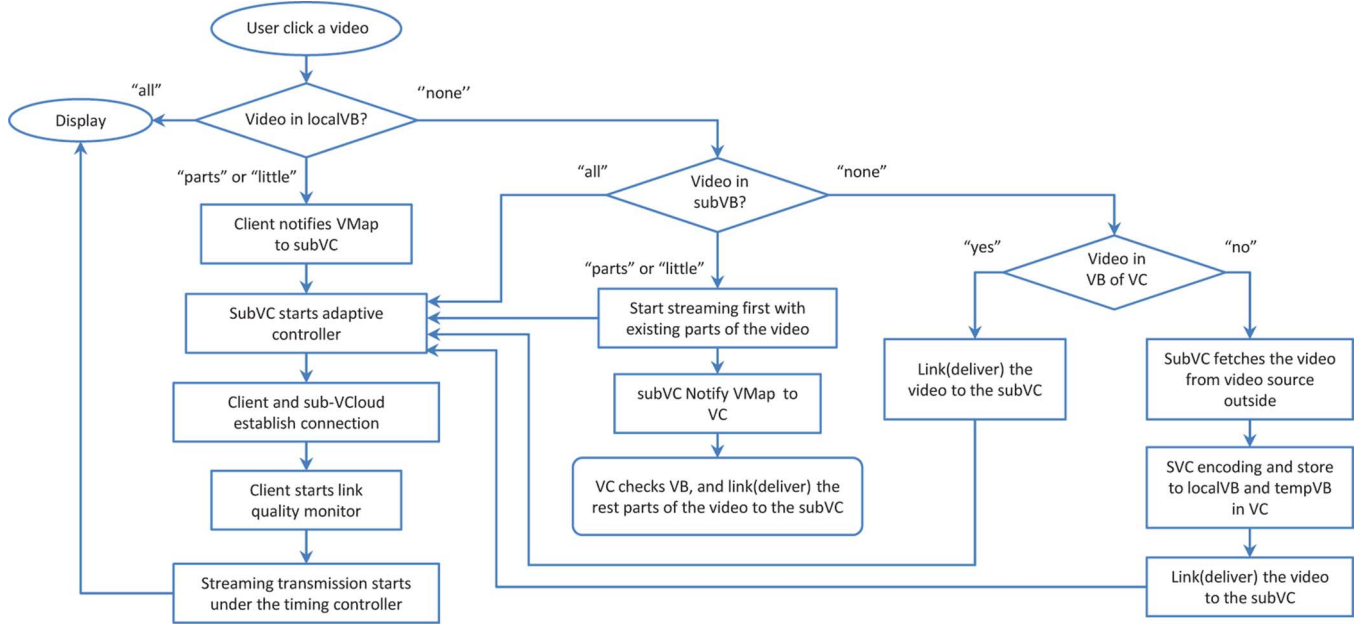
Fig. 5. Working flow of video streaming in the subVC and VC of AMES-Cloud framework.
